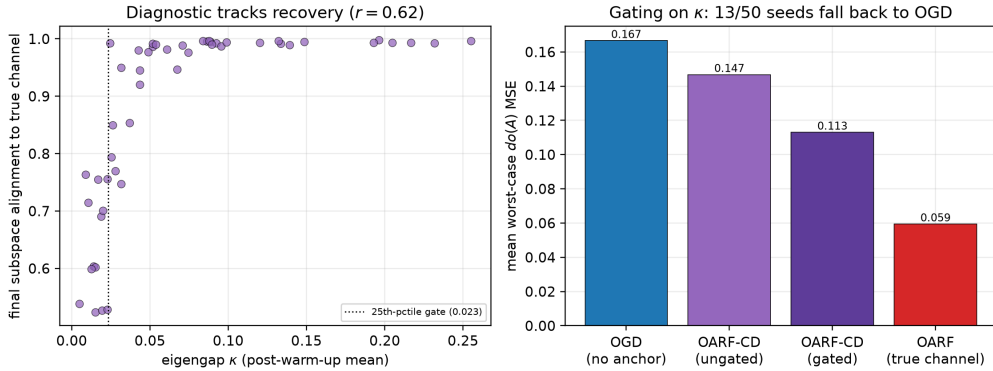
Figure 7: The eigengap diagnostic, validated. (a) Per-seed post-warm-up eigengap \kappa vs. true subspace alignment ( r = 0.62 ); the dotted line is the 25th-percentile gate. (b) Mean worst-case do( A ) MSE for OGD, ungated OARF-CD, OARF-CD gated on \kappa , and fixed-channel OARF with the true channel. Gating recovers about a quarter of the ungated learned channel’s mean worst-case error without using the ground truth.
