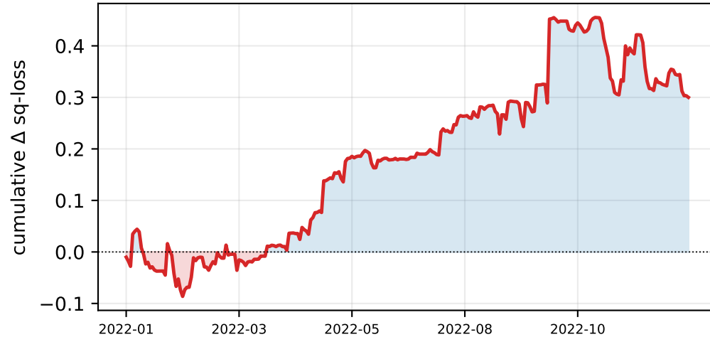
Energy shock (2022) cum. sq-loss, OARF – OGD ( < 0 : OARF better)
