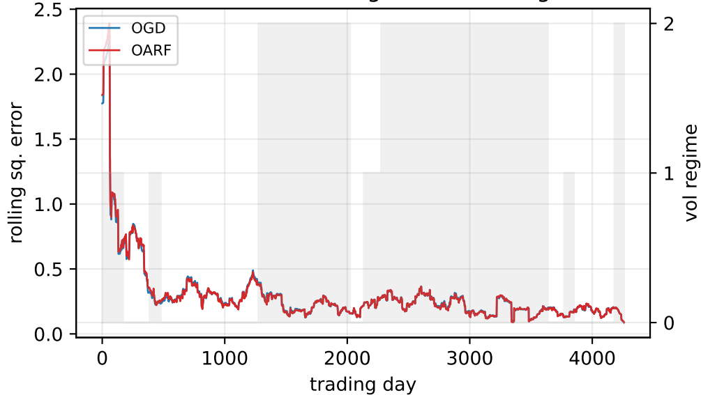
DCOILBRETEU: rolling error &amp; vol regimes
