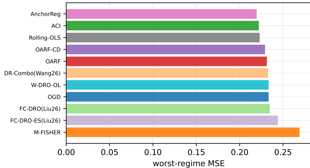
DCOILBRETEU: worst-regime MSE
