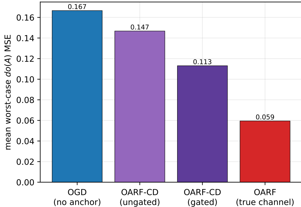
Gating on \kappa : 13/50 seeds fall back to OGD
