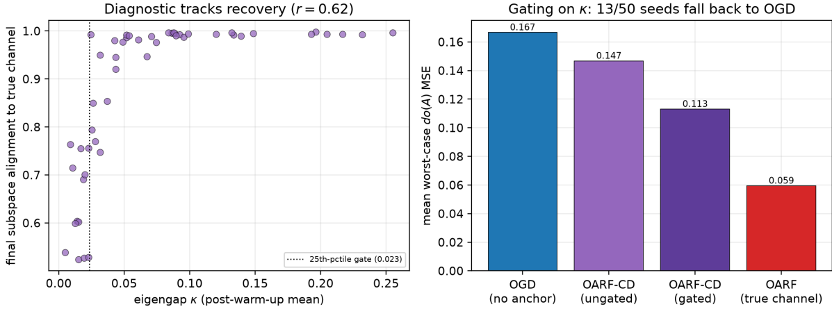
Figure 7: The eigengap diagnostic, validated. (a) Per-seed post-warm-up eigengap \kappa vs. true subspace alignment ( r = 0.62 ); the dotted line is the 25th-percentile gate. (b) Mean worst-case \text{do}(A) MSE for OGD, ungated OARF-CD, OARF-CD gated on \kappa , and fixed-channel OARF with the true channel. Gating recovers about a quarter of the ungated learned channel’s mean worst-case error without using the ground truth.
