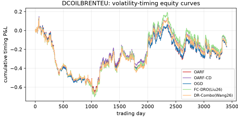
Figure 13: Brent: cumulative volatility-timing profit and loss. Differences across methods are economically small and not significant over this sample.
