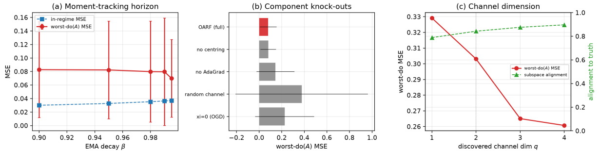
Figure 8: Ablations. (a) Sensitivity to the EMA decay \beta . (b) Component knock-outs by worst-case interventional MSE: the channel and the adaptive step are load-bearing, a random channel is worse than none. (c) Discovered-channel dimension: robustness and alignment both improve with q and are already strong at the true q = 2 (dotted).
