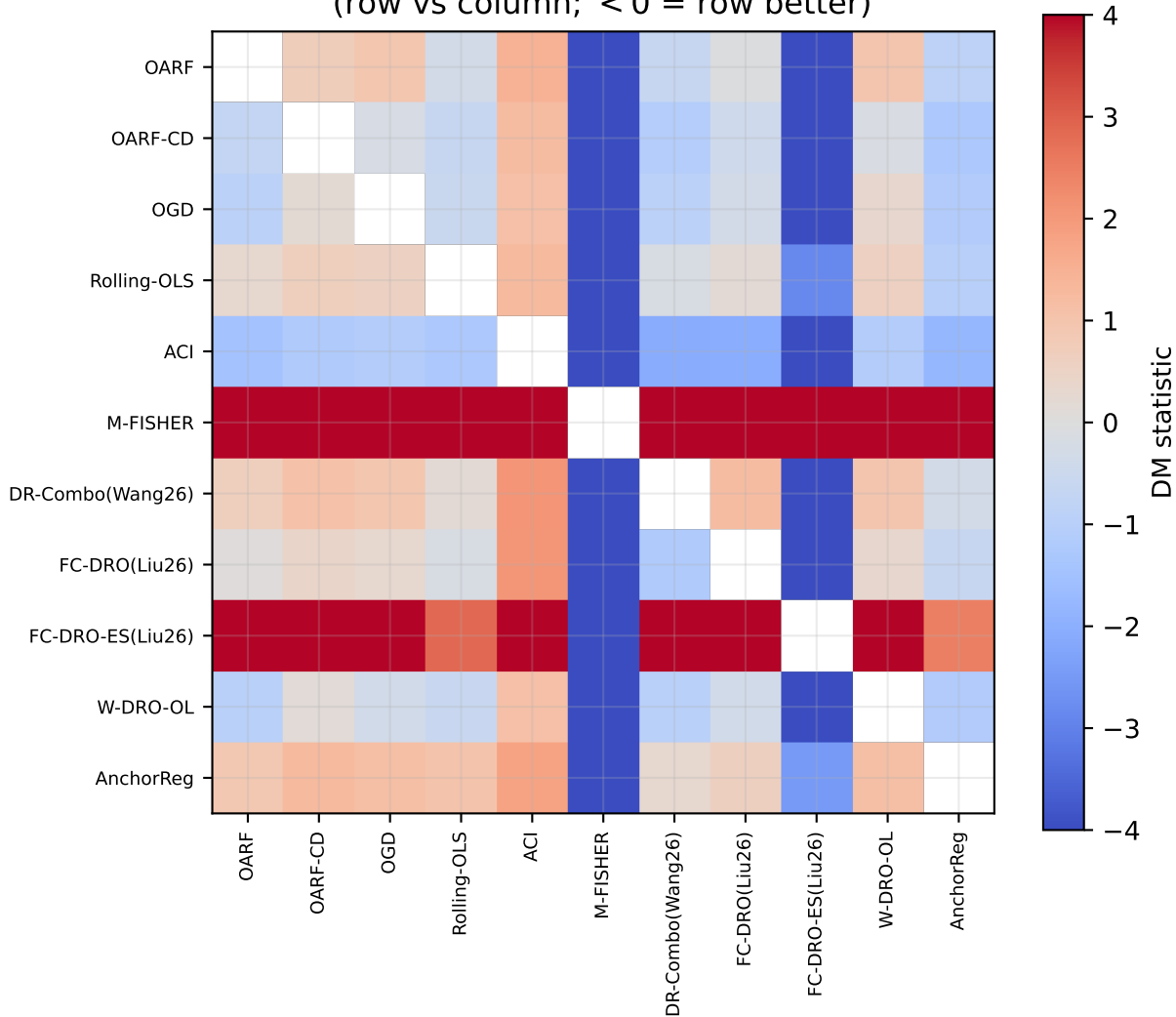
DHHNGSP: Diebold--Mariano statistic (row vs column; < 0 = row better)
