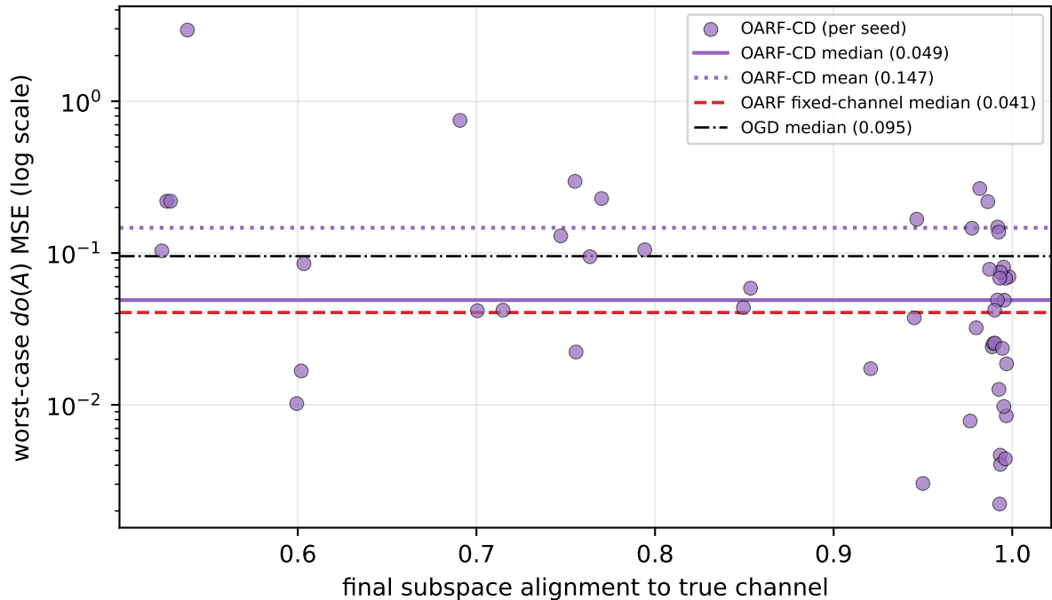
Learned channel: alignment vs robustness, per seed
