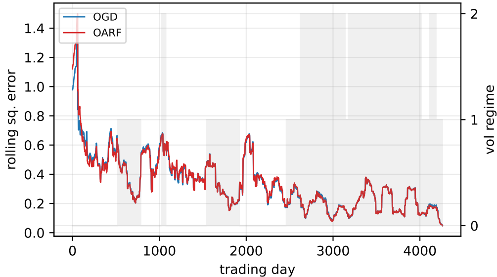
DHHNGSP: rolling error &amp; vol regimes
