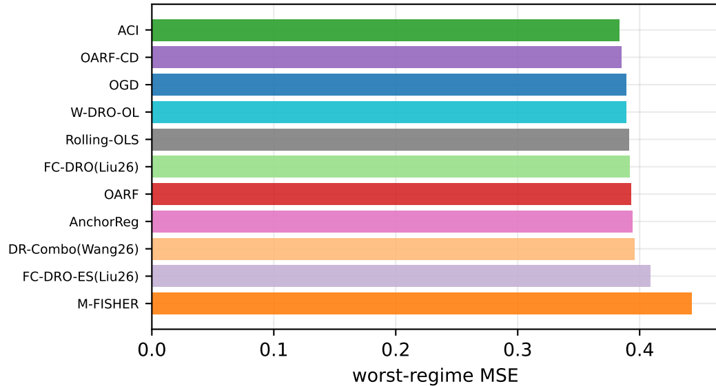
DHHNGSP: worst-regime MSE
