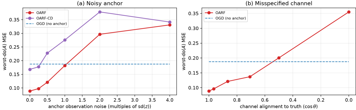
Figure 8: Stress tests of the fixed-channel method ( \text{worst-do}(A) MSE; OGD baseline dashed). (a) Increasing anchor observation noise: OARF crosses the no-anchor baseline near one standard deviation of noise. (b) Rotating the channel away from the truth: anchoring helps only while alignment \cos \theta \gtrsim 0.6 and hurts beyond it. A wrong anchor is not a benign hedge.
