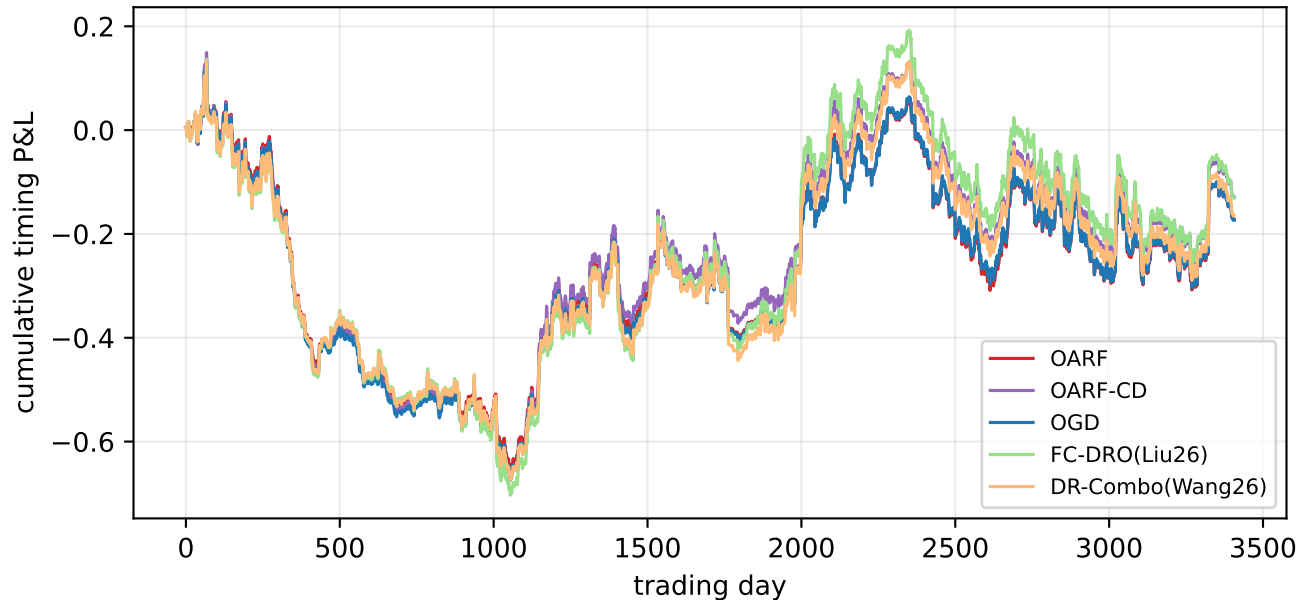
DCOILBRENTU: volatility-timing equity curves
