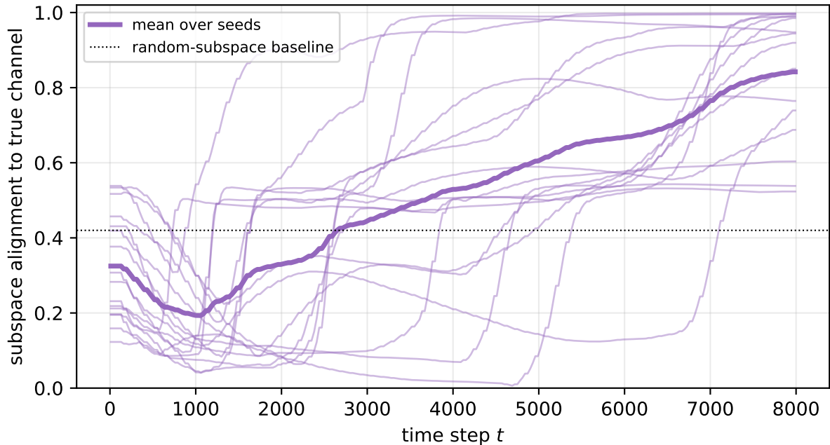
Online channel discovery (Sec 2.3): recovery over time
