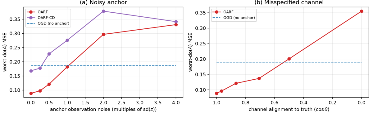
Figure 9: Stress tests of the fixed-channel method (worst-do(A) MSE; OGD baseline dashed). (a) Increasing anchor observation noise: OARF crosses the no-anchor baseline near one standard deviation of noise. (b) Rotating the channel away from the truth: anchoring helps while alignment \cos \theta \gtrsim 0.6 and hurts beyond that point.
