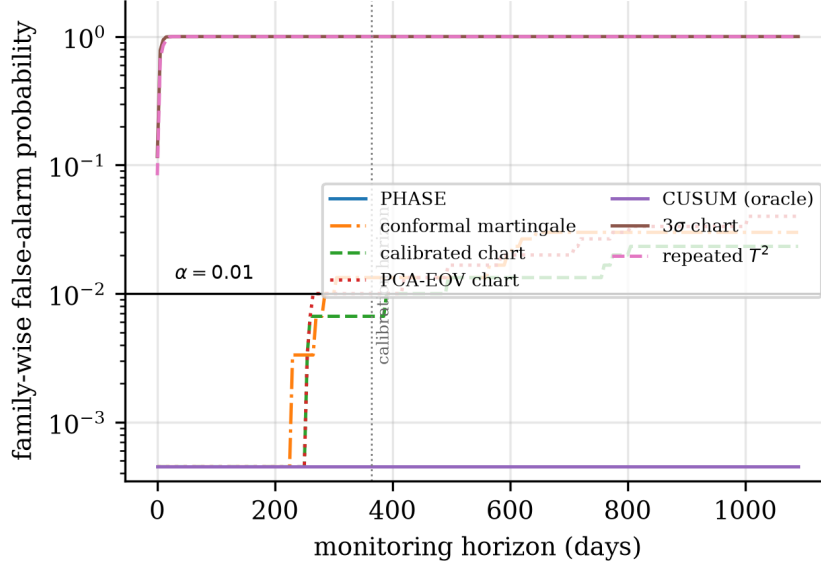
Figure 3: Family-wise false-alarm probability as a function of monitoring horizon, from 300 undamaged four-year records. Curves for PHASE and the oracle CUSUM lie on the axis floor (no false alarm observed). The calibrated chart controls error only up to the horizon for which it was tuned.
