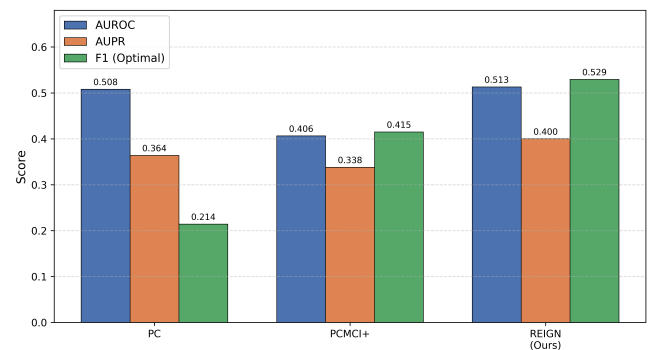
Figure 5. Quantitative performance comparison (AUROC, AUPR, F1) across all currently evaluated models on the VAR-Regime dataset. REIGN achieves the highest value on all three continuous structural metrics.
