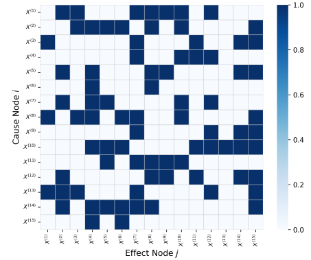
Figure 4. Global ground-truth causal graph \mathcal{G} (15 nodes, 81 edges) shown as a binary adjacency heatmap. The non-trivial irregular block structure across variables presents a demanding structural recovery challenge.
