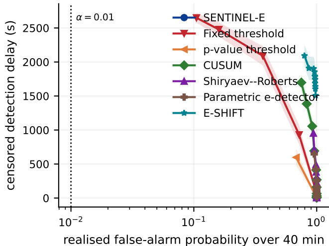
(a) delay vs false-alarm probability
