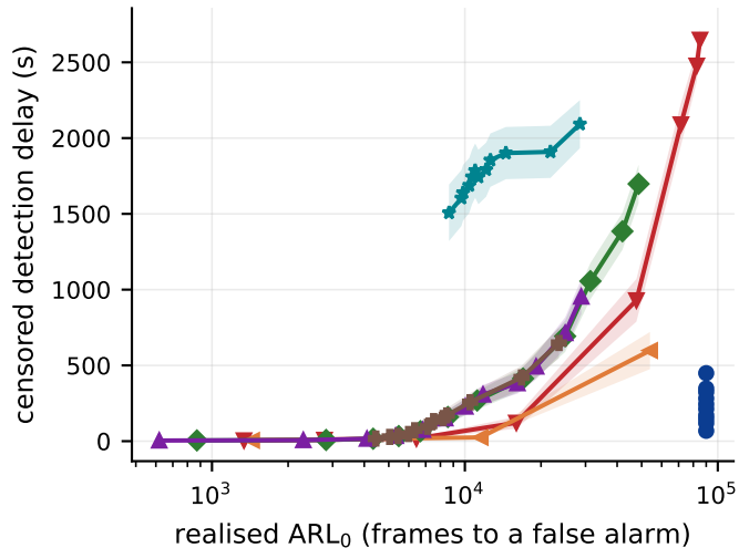
(b) delay vs mean time between false alarms
