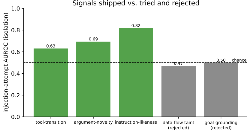
Fig. 8 Injection-attempt AUROC (in isolation) of the three shipped signals and the two rejected ones. The rejected signals sit at or below the chance line even with the capable agent; Section 7.3 explains why lexical proxies for provenance and goal-grounding are too coarse.
