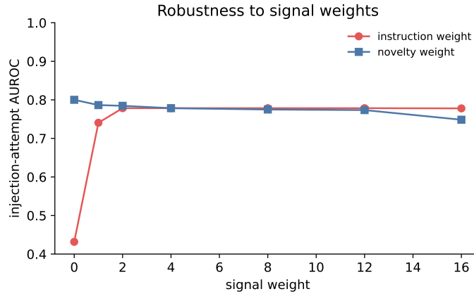
Fig. 7 Robustness of injection-attempt AUROC to the novelty and instruction signal weights. Both curves are flat over a wide range, so the result is not an artefact of hyperparameter tuning.
