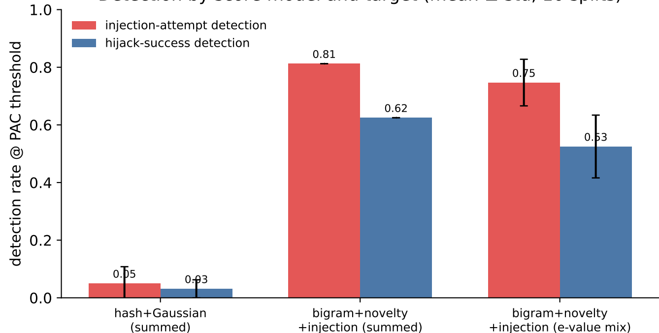
Detection by score model and target (mean \pm std, 10 splits)
