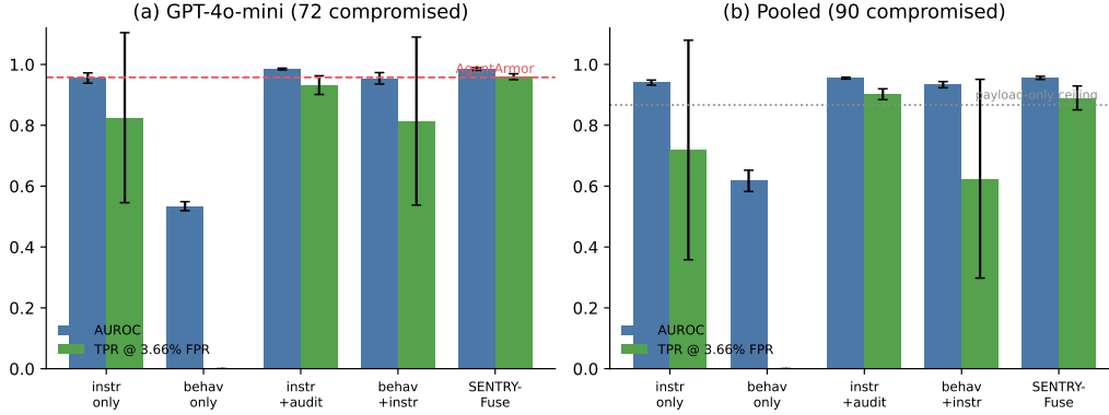
Figure 1: Fusion ablation. (a) On GPT-4o-mini the four-signal fusion exceeds the strongest published trace-only operating point (dashed). (b) Pooled, the fused detectors exceed the payload-visibility ceiling (dotted), which no observation-only detector can. Error bars are one standard deviation over ten seeds.
