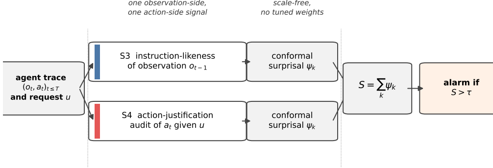
Figure 1: Overview of SENTRY-Fuse. Two signals are computed per action, one from each evidence channel: the observation channel (S3) asks whether untrusted content is behaving like an instruction, while the action channel (S4) asks whether the agent’s behaviour serves the user’s request. Each raw score is mapped to a conformal tail surprisal against a benign calibration split, which makes the heterogeneous signals commensurable at a far finer resolution than the excess-over-maximum alternative of Proposition 1, which collapses a whole class to a point. The surprisals are summed and thresholded; on an alarm the largest term, \arg \max_k \psi_k , names the signal that fired, which gives the operator an actionable reason rather than a bare alert.
