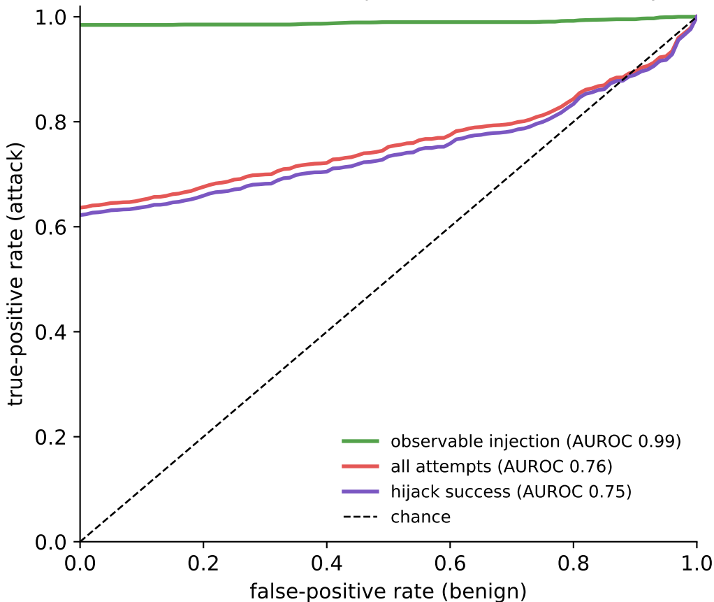
ROC on real held-out trajectories (mean of 10 splits)
