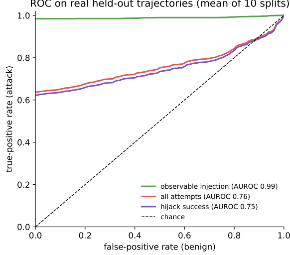
Fig. 5 ROC of the shipped three-signal model on real held-out trajectories, averaged over the ten splits (AUROC annotated). On the observable-injection subset the monitor is near-perfect; the all-attempts and hijack-success curves are bounded away from the top-left corner entirely by the 70/198 attacks whose payload never enters the monitored trace (Section 4.4), not by false negatives on visible injections.
