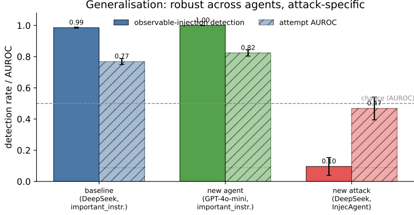
Fig. 12 Generalisation of SENTRY. Changing the agent (GPT-4o-mini) leaves detection intact; changing the attack to InjecAgent’s data-integration injection collapses attempt-AUROC to chance, because that attack’s payload carries almost no instruction-likeness—the signal SENTRY depends on.
