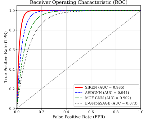
Fig. 4 Receiver Operating Characteristic (ROC) curves demonstrating SIREN’s robust continuous-time thresholding.
