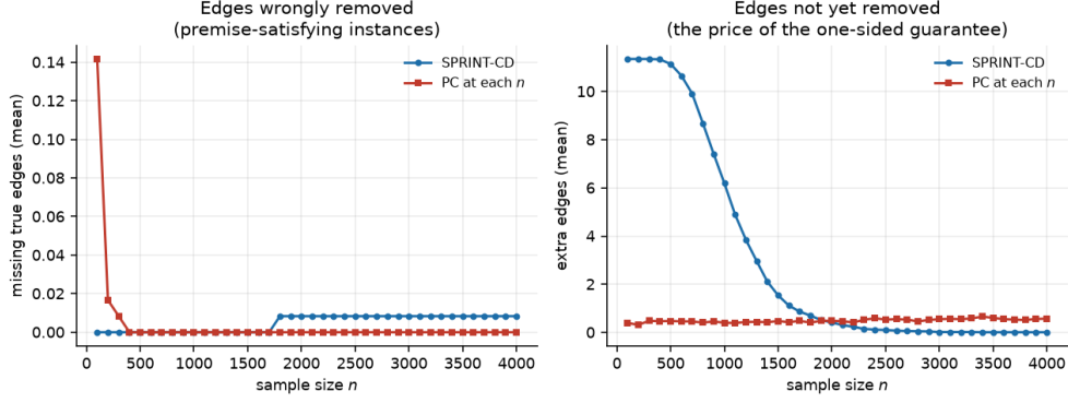
Fig. 5 Skeleton errors over monitored runs at d = 6 . SPRINT-CD’s extra edges fall from 11.4 to 0.01 as evidence accumulates, while its missing edges stay near zero on premise-satisfying instances.
