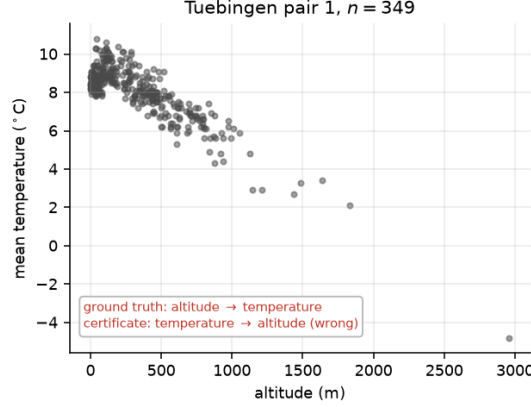
Fig. 11 A worked example, one of the 14 pairs on which the direction certificate commits: Tübingen pair 1 (altitude versus mean temperature, n = 349 ). Here it commits and gets it wrong, with no indication in its output that this instance differs from a correct one.
