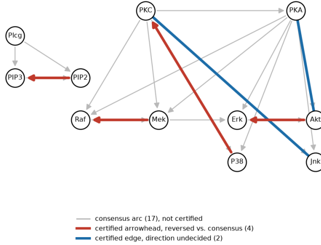
Fig. 10 A worked example, not an aggregate: CERT-CD’s certified output on the Sachs network, drawn against the published 17-arc consensus (grey). Of the 6 certified edges, 4 also carry a certified arrowhead, and every one of those 4 points opposite the consensus arc on that pair (red); the remaining 2 certified edges (Akt–PKA, PKC–Jnk) stay undirected (blue).
