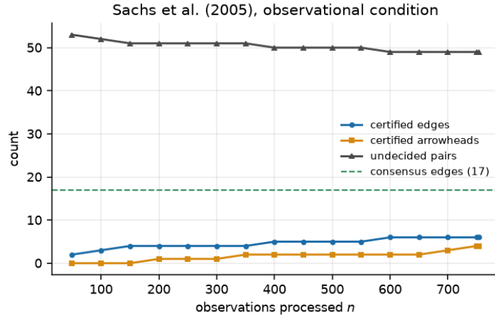
Fig. 13 CERT-CD on the Sachs observational sample. Certified edges accumulate slowly and the undecided set stays large: at n = 753 , 49 of 55 pairs remain undecided.
