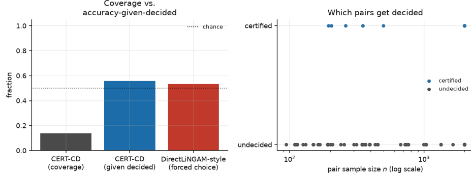
Fig. 12 The direction certificate on 102 Tübingen cause-effect pairs. Left: coverage (fraction of pairs certified), weighted accuracy conditional on certification, and the forced-choice comparison statistic’s weighted accuracy, against chance. Right: which pairs get decided, by sample size.
