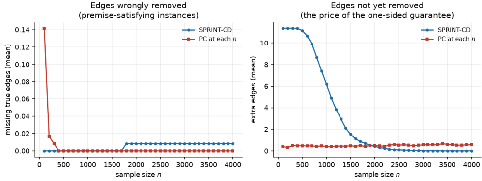
Fig. 4 Skeleton errors over monitored runs at d = 6 . SPRINT-CD’s extra edges fall from 11.4 to 0.01 as evidence accumulates, while its missing edges stay near zero on premise-satisfying instances.
