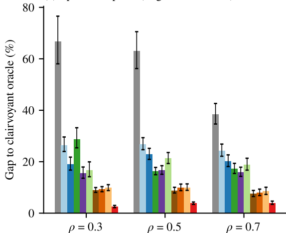
(a) Spatio-temporal (migration allowed)
