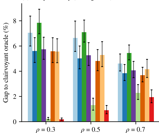
(b) Temporal-only (no migration)
