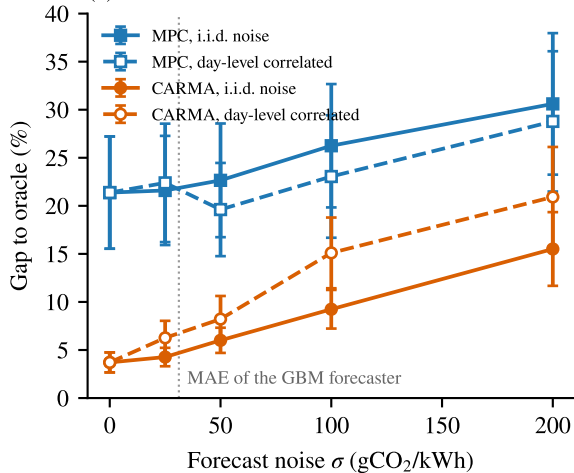
(a) Carbon-forecast error
