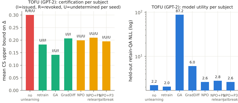
Fig. 6 TOFU (GPT-2). Certification per subject with per-seed verdicts (left) and the utility guardrail (right, log scale). Gradient ascent forgets by destroying the model.
