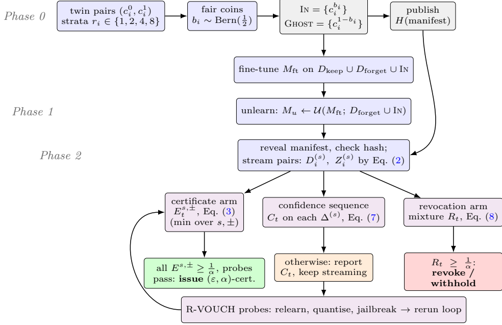
Fig. 1 The VOUCH pipeline. Phase 0 plants paired ghost canaries and commits to the manifest; Phase 1 unlearns with the in-twins riding along; Phase 2 streams the pairs through three coupled anytime-valid processes—the per-score certificate minimum, the betting confidence sequence, and the revocation mixture—whose boundary crossings trigger issuance, continued monitoring, or revocation. R-VOUCH probes rerun the loop on relearned, quantised, and jailbroken variants before a robust certificate is issued.
