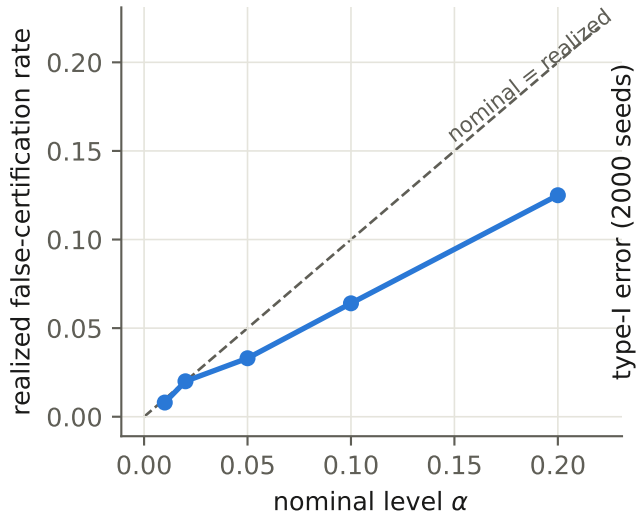
VOUCH is conservative under adversarial optional stopping
