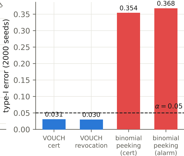
Anytime validity vs fixed- n peeking
