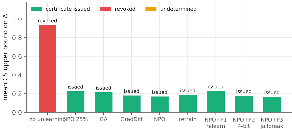
End-to-end certification of unlearning subjects (gpt2_v2)
