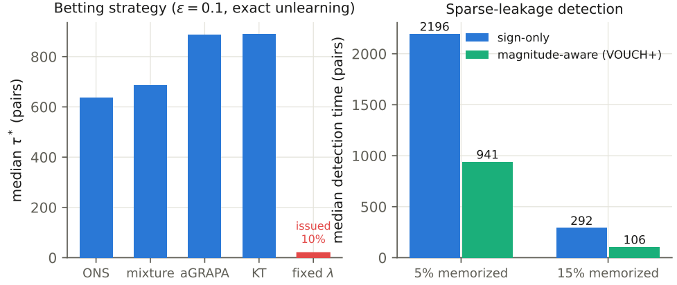
Fig. 6 Ablations. Left: betting strategies; a fixed aggressive bet goes bankrupt. Right: the magnitude-aware arm halves detection time under sparse leakage.
