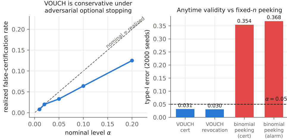
Fig. 1 Anytime validity. Left: the realised false-certification rate lies below the nominal level at every \alpha under adversarial optional stopping. Right: a fixed- n binomial test used with peeking inflates its error sevenfold; VOUCH does not.
