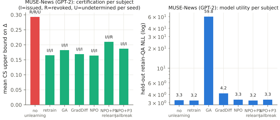
Fig. 5 MUSE-News (GPT-2, 512 pairs). The genuine unlearning methods certify, the unlearned model is revoked, and gradient ascent again destroys utility.
