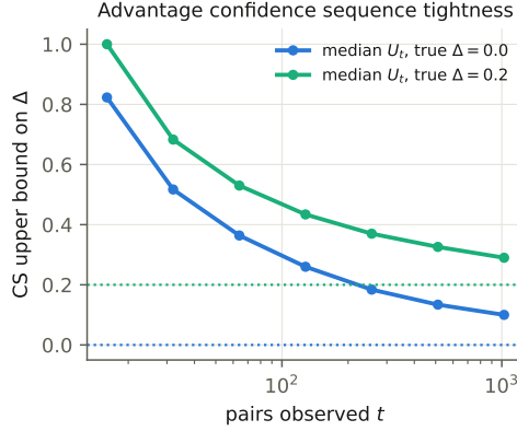
Fig. 3 Tightness. The anytime confidence-sequence upper bound on \Delta shrinks with the number of pairs observed, under \Delta = 0 and \Delta = 0.2 .
