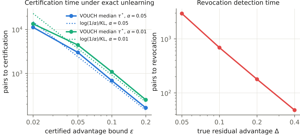
Fig. 2 Power. Left: median certification time versus \epsilon , against the information limit \log(1/\alpha)/KL . Right: revocation detection time versus the true residual advantage.
