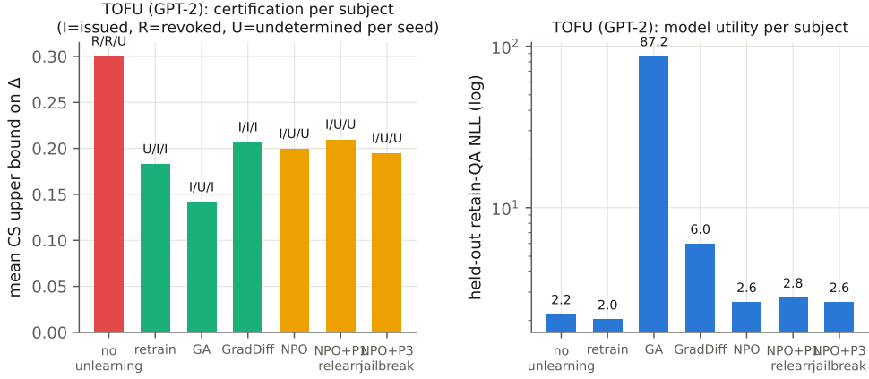
Fig. 4 TOFU (GPT-2). Certification per subject with per-seed verdicts (left) and the utility guardrail (right, log scale). Gradient ascent forgets by destroying the model.
