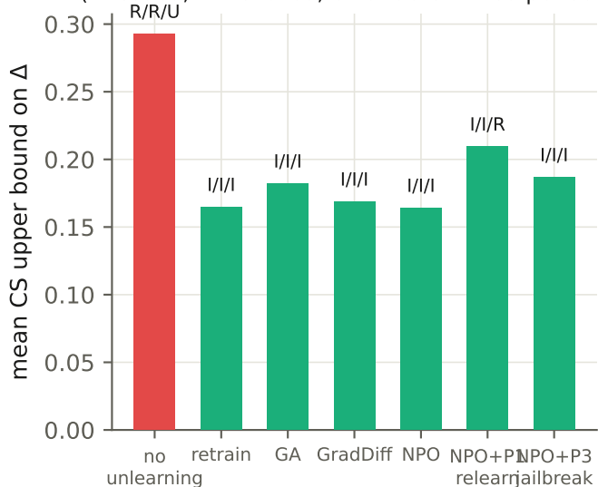
MUSE-News (GPT-2): certification per subject (I=issued, R=revoked, U=undetermined per seed)
