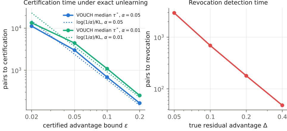
Fig. 3 Power. Left: median certification time versus \varepsilon , against the information limit \log(1/\alpha)/KL . Right: revocation detection time versus the true residual advantage.
