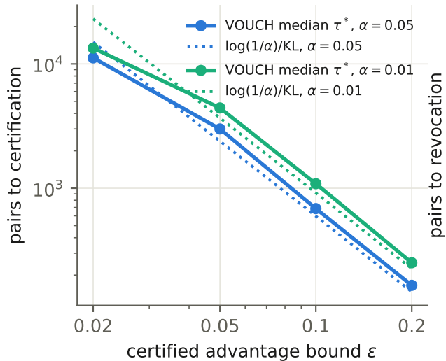
Certification time under exact unlearning
