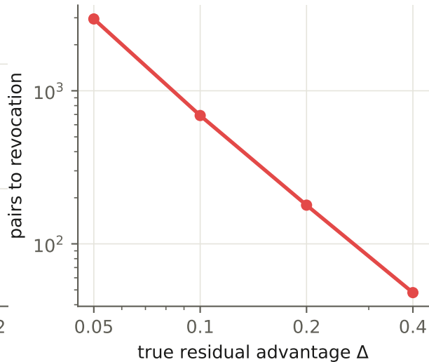
Revocation detection time
