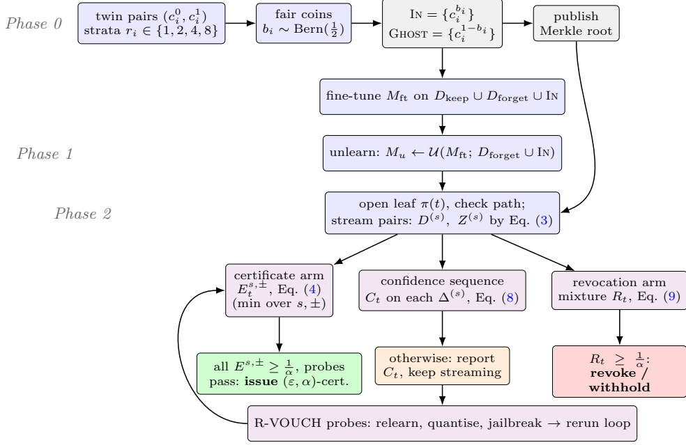
Fig. 1 The VOUCH pipeline. Phase 0 plants paired ghost canaries and commits to the manifest as a Merkle tree ; Phase 1 unlearns with the in-twins riding along; Phase 2 opens one leaf at a time in a committed random order and streams the pairs through three coupled anytime-valid processes—the per-score certificate minimum, the betting confidence sequence, and the revocation mixture—whose boundary crossings trigger issuance, continued monitoring, or revocation. R-VOUCH probes rerun the loop on relearned, quantised, and jailbroken variants before a robust certificate is issued.
