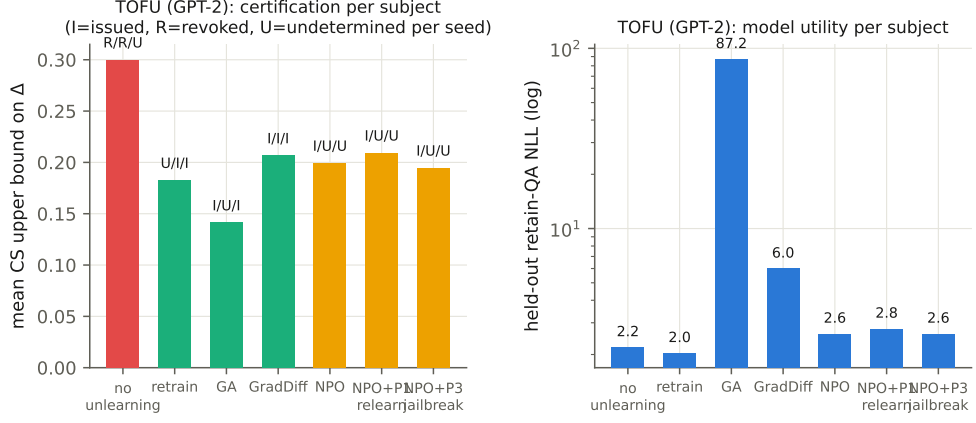
Fig. 6 TOFU (GPT-2). Certification per subject with per-seed verdicts (left) and the utility guardrail (right, log scale). Gradient ascent forgets by earns its certificate while destroying the model held-out performance .
