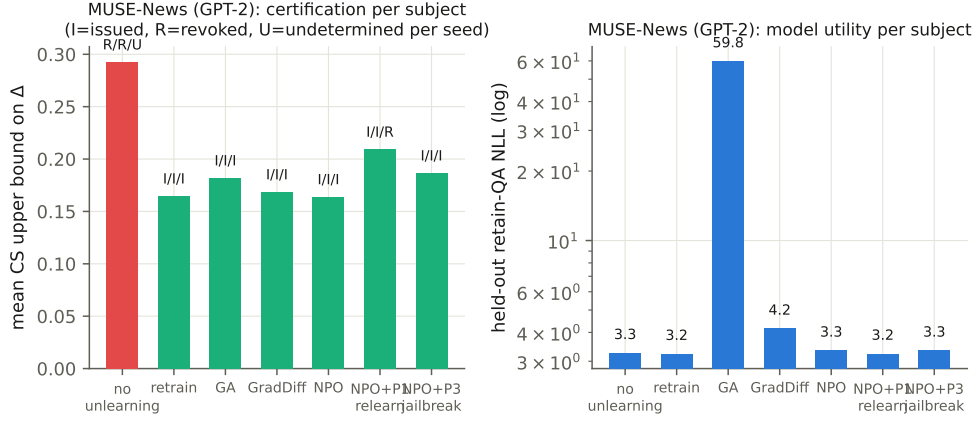
Fig. 7 MUSE-News (GPT-2, 512 pairs). The genuine unlearning methods certify, the unlearned model is revoked, and gradient ascent again destroys utility.
