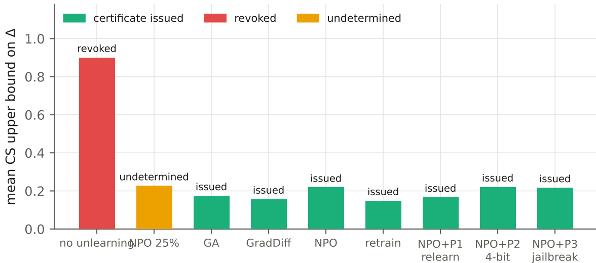
End-to-end certification of unlearning subjects (tiny)
