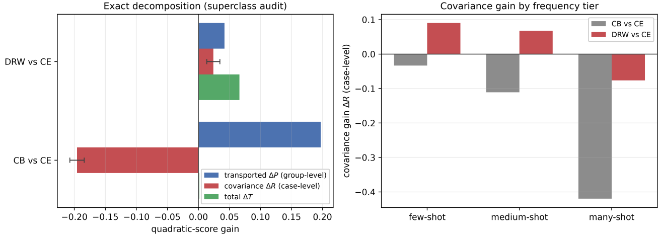
Figure 8. The same attribution transfers to a second task. Left: exact decomposition at the superclass audit. The CB total gain (green) is visually almost absent at +0.00143 while its two channels reach \pm 0.2 – a near-zero aggregate score concealing two large opposing effects. DRW’s smaller total is genuinely split between both channels. Error bars are 95% Hájek intervals on \widehat{\Delta R} . Right: the covariance channel by training-frequency tier, showing that DRW’s genuine per-instance gain is concentrated on rare classes and negative on the head.
