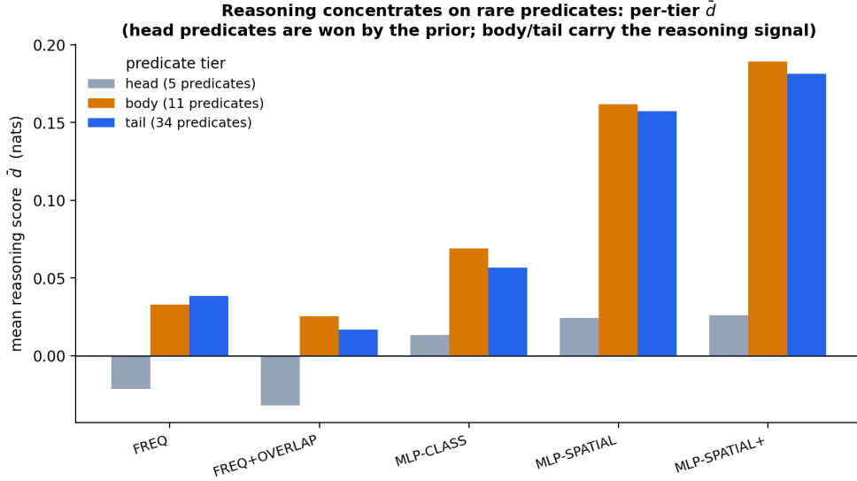
Fig. 9 Reasoning concentrates on rare predicates. Mean reasoning score \bar{d} per predicate tier. Head predicates are won by the prior; the body and tail carry the reasoning signal, and it grows with spatial capacity.
