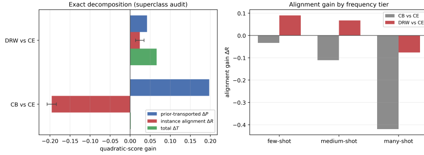
Figure G.7: The same attribution transfers to a second task. Left: exact decomposition at the superclass audit. The CB total gain (green) is visually almost absent at +0.00143 while its two channels reach \pm 0.2 – a near-zero aggregate score concealing two large opposing effects. DRW’s smaller total is genuinely split between both channels. Error bars are 95% Hájek intervals on \widehat{\Delta R} . Right: the covariance channel by training-frequency tier, showing that DRW’s genuine per-instance gain is concentrated on rare classes and negative on the head.
