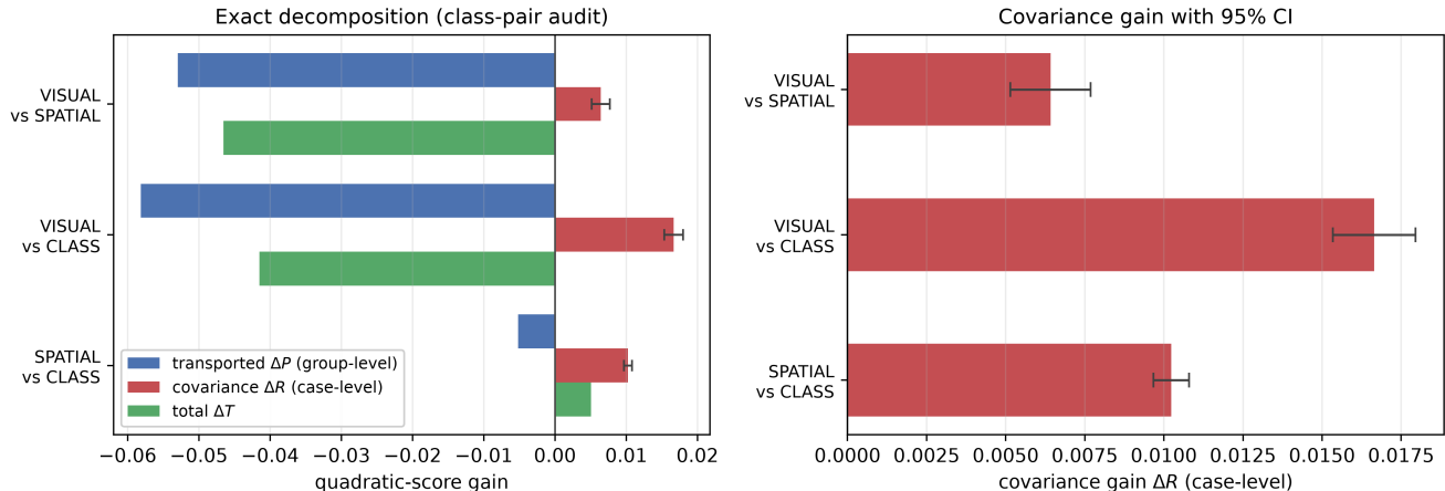
Figure 7. Pixels beat geometry on covariance while losing on the aggregate. Left: the exact decomposition for the three matched-subsample pairs. Both comparisons involving the CLIP model have strongly negative totals (green) driven entirely by the transported channel (blue), while their covariance channel (red) is positive in every case. Right: the covariance channel alone, with 95% image-clustered intervals. Replacing box geometry with real image content raises within-group covariance from 0.01023 to 0.01665 over the same class-only baseline.
