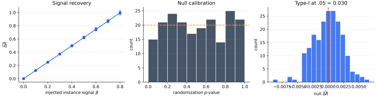
Figure 4. Controlled validation. WAGER recovers injected within-cell signal monotonically (mean \pm one standard deviation), produces approximately uniform null randomization p -values, and controls type-I error in 200 null runs.
