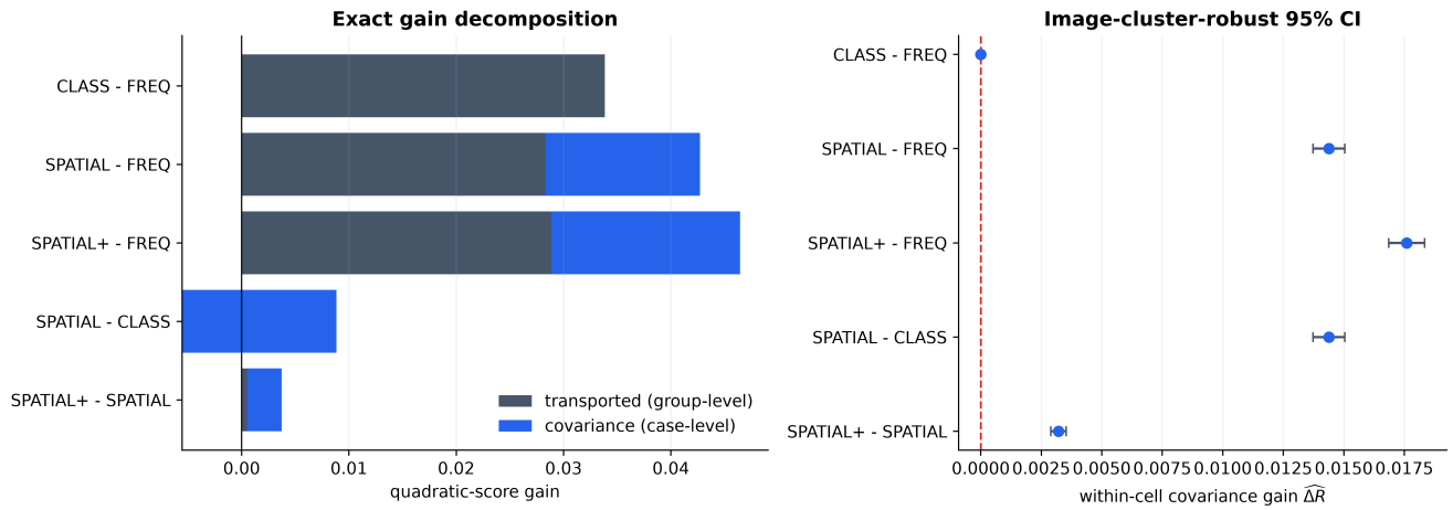
Figure 6. Direct model-pair attribution. Left: exact decomposition of each positive gain into transported and within-group covariance components (the negative prior term for SPATIAL–CLASS extends left of zero). Right: primary covariance estimates with image-cluster-robust intervals.
