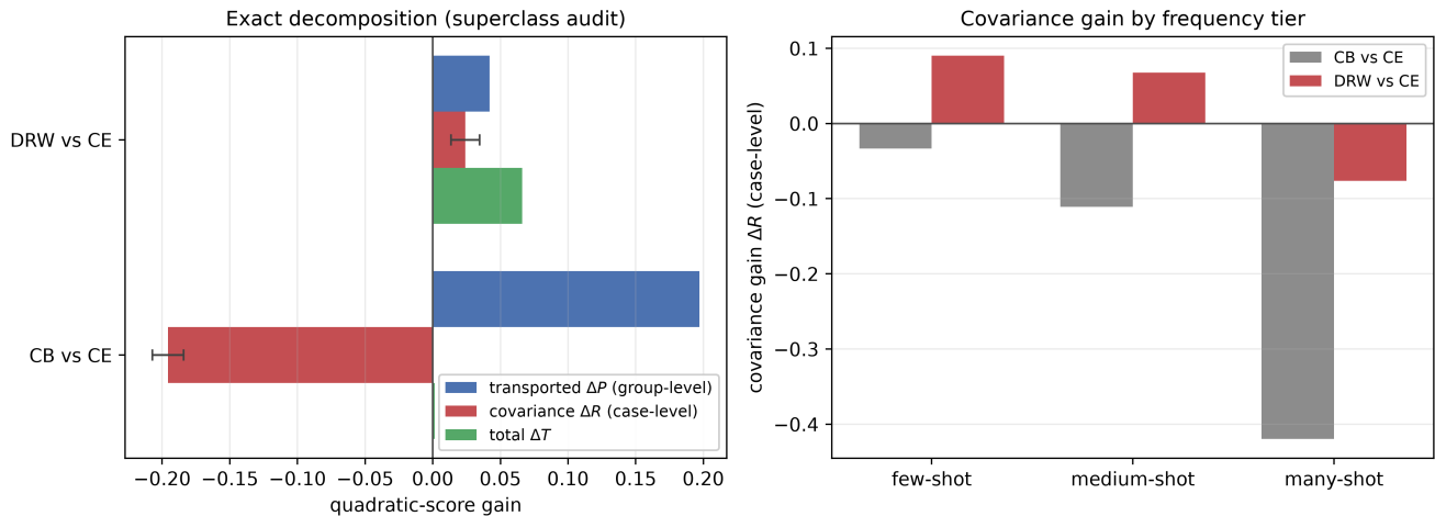
Figure 8. The same attribution transfers to a second task. Left: exact decomposition at the superclass audit. The CB total gain (green) is visually almost absent at +0.00143 while its two channels reach \pm 0.2 – a near-zero aggregate score concealing two large opposing effects. DRW’s smaller total is genuinely split between both channels. Error bars are 95% Hájek intervals on \widehat{\Delta R} . Right: the covariance channel by training-frequency tier, showing that DRW’s genuine per-instance gain is concentrated on rare classes and negative on the head.
