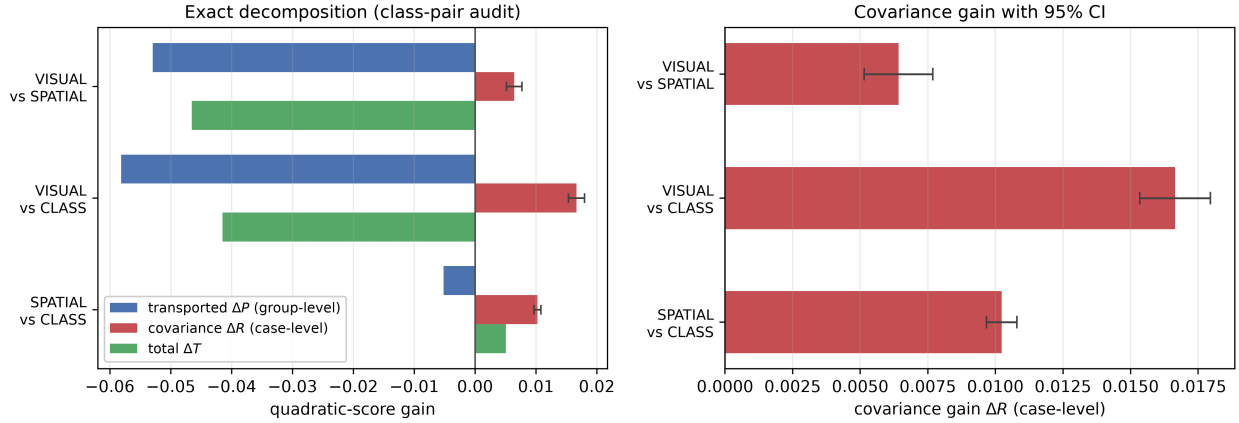
Figure 5: Pixels beat geometry on covariance while losing on the aggregate. Left: the exact decomposition for the three matched-subsample pairs. Both comparisons involving the CLIP model have strongly negative totals (green) driven entirely by the transported channel (blue), while their covariance channel (red) is positive in every case. Right: the covariance channel alone, with 95% image-clustered intervals. Replacing box geometry with real image content raises within-group covariance from 0.01023 to 0.01665 over the same class-only baseline.
