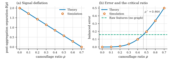
Fig. 1 Theory versus simulation. (a) Post-aggregation separation decays linearly in \rho exactly as Proposition 4 predicts. (b) Balanced error against the attribute-only baseline; the predicted critical ratio \rho^* = 0.464 coincides with the crossing point.
