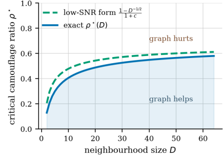
Figure 2. Critical camouflage ratio against neighbourhood size. Below the curve the graph improves on raw features; above it the graph is actively harmful. The closed form is the noise-dominated limit of the exact crossover.
