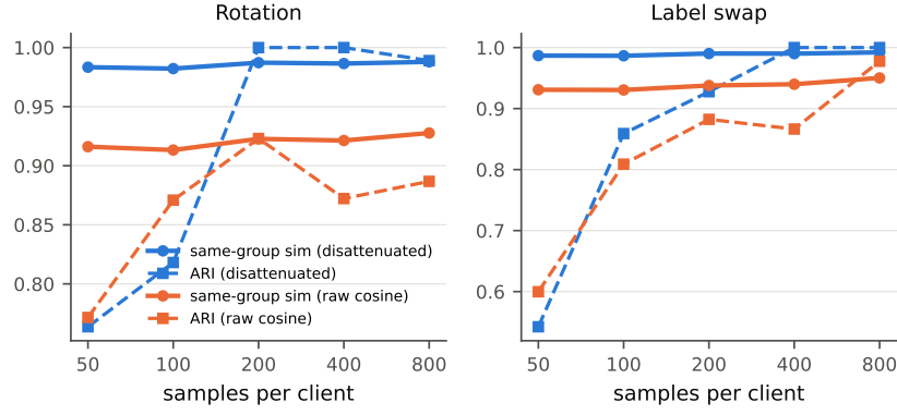
Fig. B1: Same-group similarity (solid) and ARI (dashed) as a function of the client size. Blue: disattenuated; orange: raw cosine.
