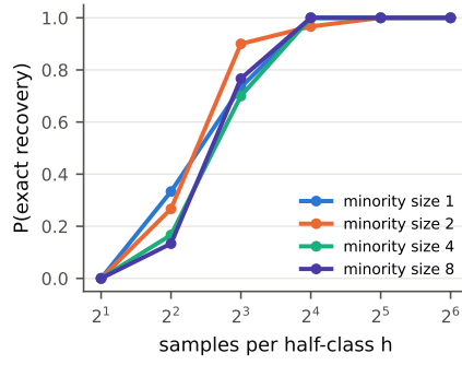
Fig. B2: Synthetic validation of Corollary 1: exact recovery of a minority group does not depend on its size.
