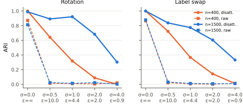
Fig. 1: Clustering quality under (\varepsilon, 10^{-5}) -DP signatures. Solid: DisCo-CFL; dashed: raw cosine. Orange: 400 samples per client; blue: 1,500.
