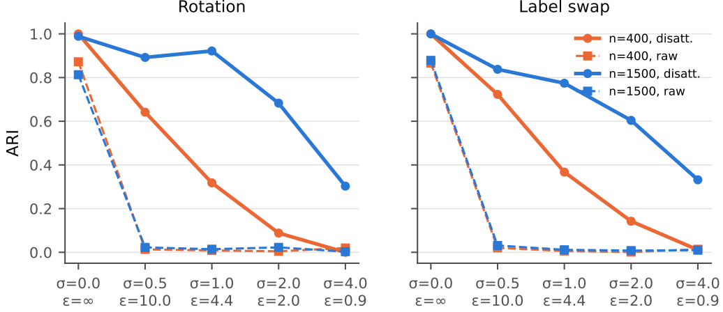
Figure 1: Clustering quality under (\epsilon, 10^{-5}) -DP signatures. Solid: DisCo-CFL; dashed: raw cosine. Orange: 400 samples per client; blue: 1,500.
