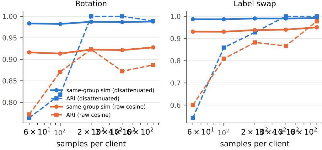
Figure 4: Same-group similarity (solid) and ARI (dashed) as a function of the client size. Blue: disattenuated; orange: raw cosine.
