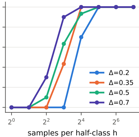
full support: exact recovery
