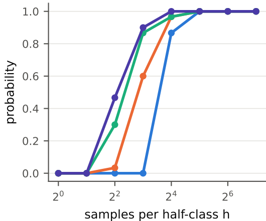
random class supports: safe & maximal
