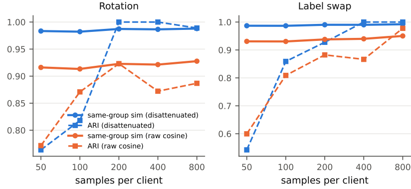
Fig. C1: Same-group similarity (solid) and ARI (dashed) as a function of the client size. Blue: disattenuated; orange: raw cosine.
