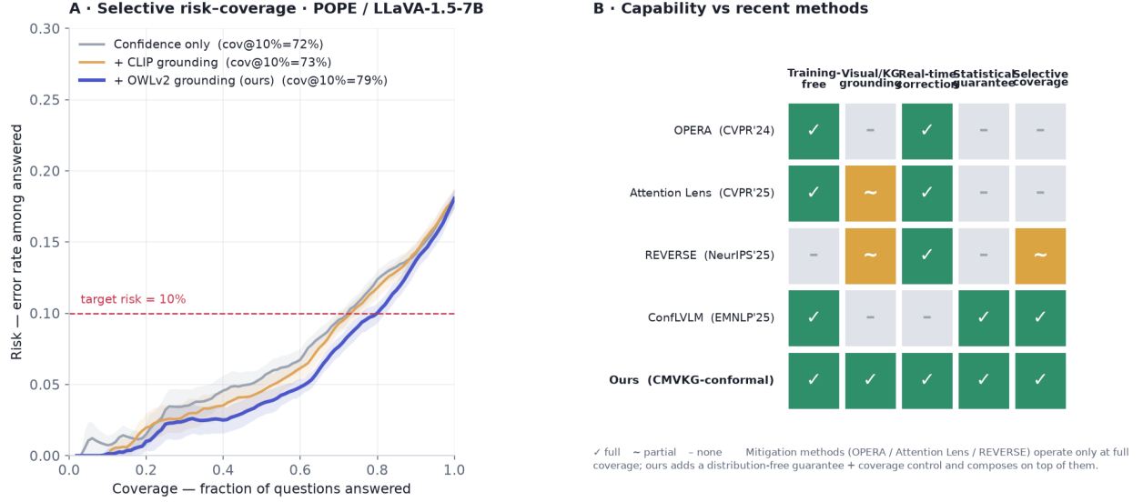
Figure 6: (A) Risk-coverage on POPE for the score variants. (B) Capability comparison with recent methods. Mitigation approaches change the base model but provide no guarantee; existing conformal approaches guarantee but only remove or abstain. Our layer composes on top of mitigation decoders (§5).
