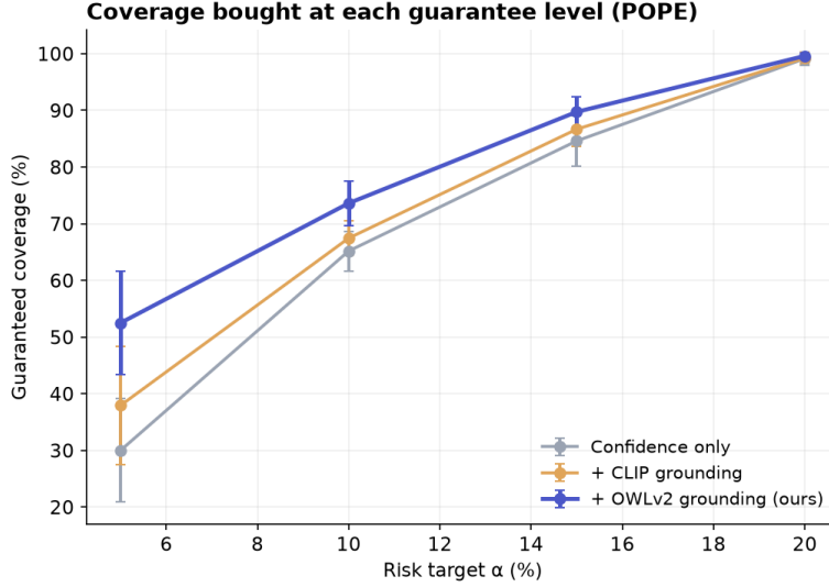
Figure 3: Certified coverage as a function of the risk target. The grounded score dominates at every level and the margin widens as \alpha tightens; at \alpha = 0.05 it nearly doubles coverage. Error bars are one standard deviation over splits.
